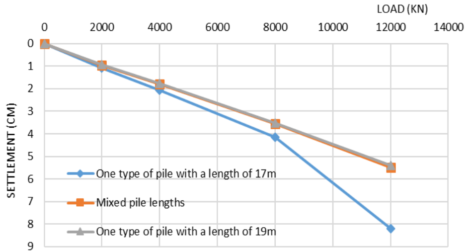
Figure 6. Load-settlement relationship for the 4-pile foundation option.
