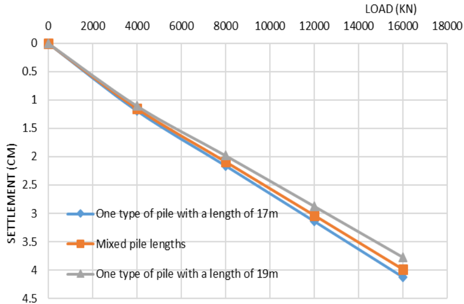
Figure 7. Load-settlement relationship for the 9-pile foundation option.
