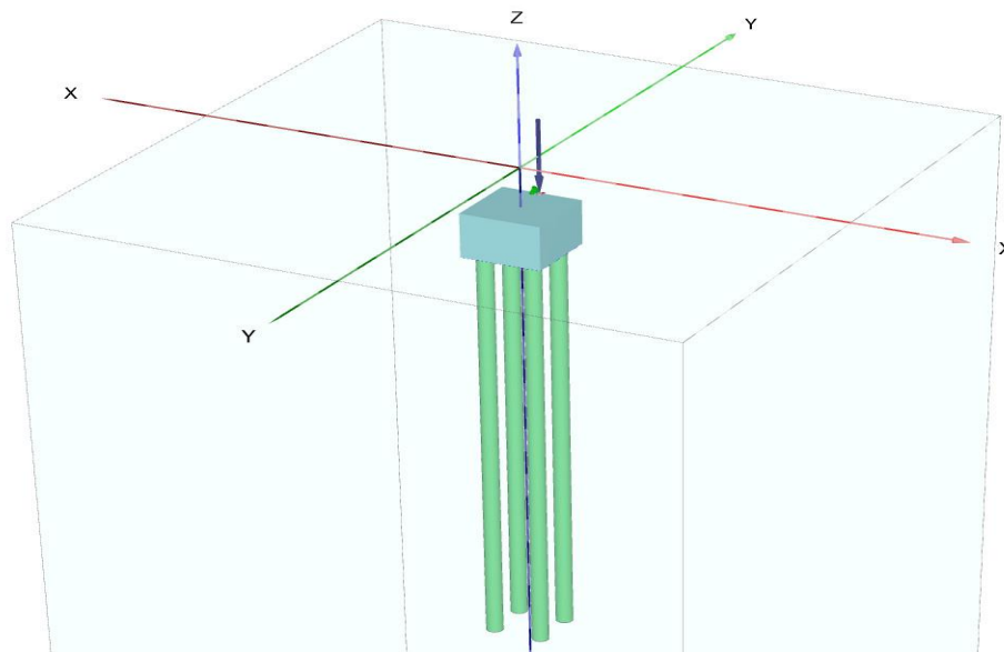
Figure 2. Model of pile foundation using Plaxis 3D Foundation V.22.
