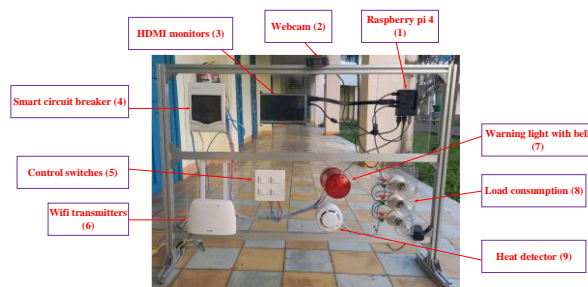
Figure 11. Actual results of the whole system.
