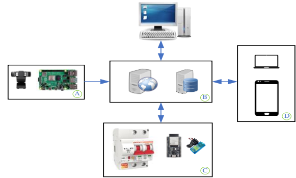
Figure 5. Schematic diagram of online monitoring structure for a distribution power system based on image processing and IoT.
