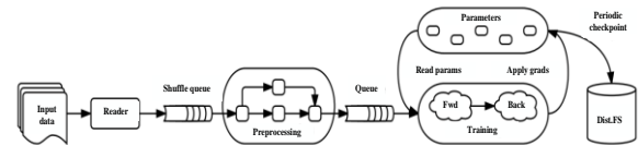
Figure 2. Data flow chart for the training process.
