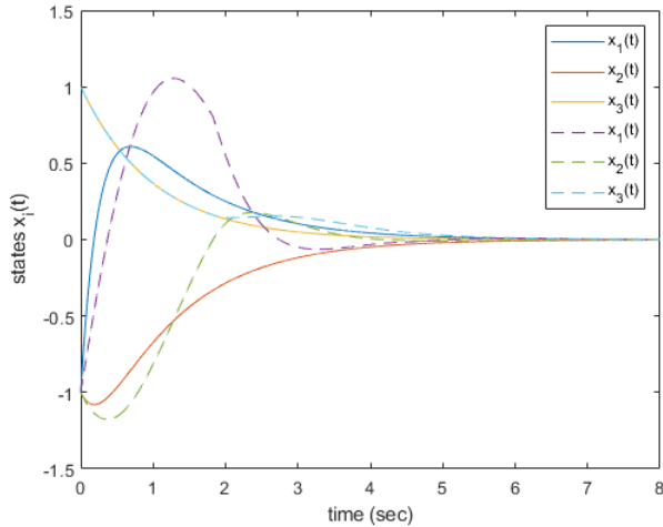
Fig. 3. Trajectories of the closed-loop three tanks system with two kinds of controllers
