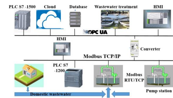
Figure 3. Applying industrial network to manage wastewater treatment system of Quy Nhon city
