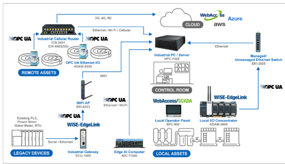
Figure 7. Wastewater treatment plant system diagram.
