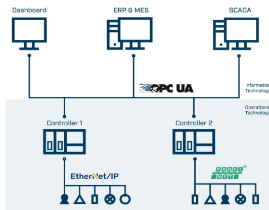
Figure 5. Ethernet industrial communication protocol.
