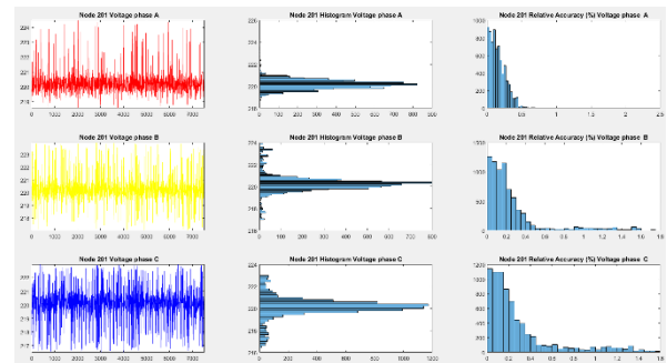
Figure 6. Voltage analysis in Node 201
