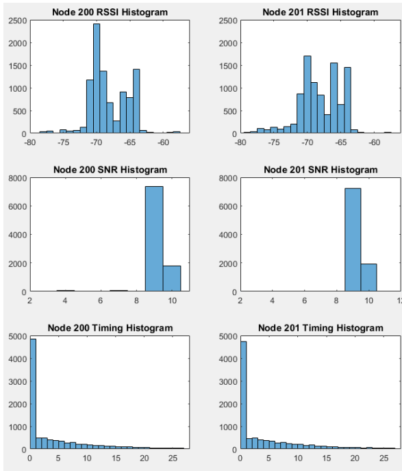
Figure 17. Histogram of RSSI, SNR and Timing values in Case2
