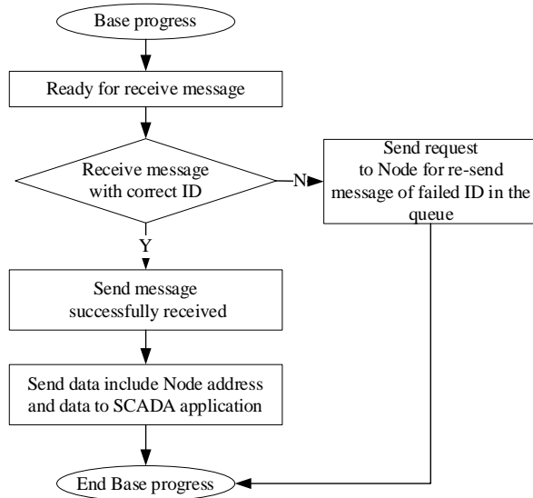
Figure 9. Base general algorithm flowchart
