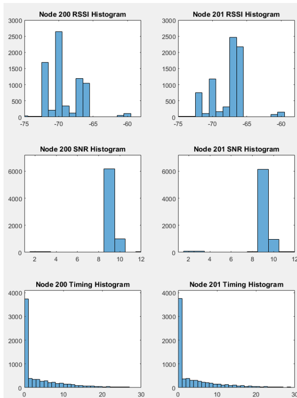
Figure 14. Histogram of RSSI, SNR and Timing values in Case1
