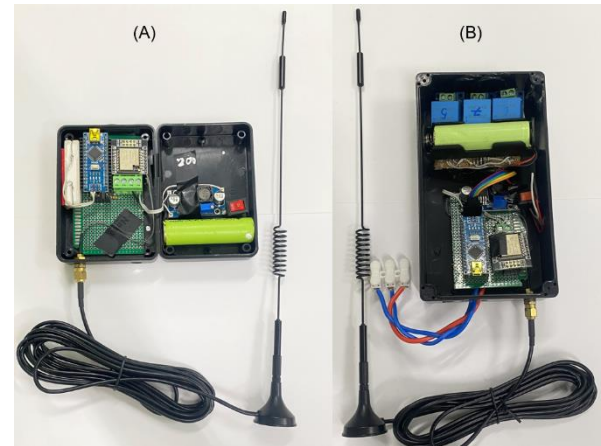
Figure 8. Intermediate node (A) Data collection node (B)
