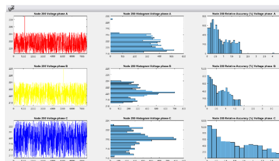
Figure 4. Voltage analysis in Node 200
