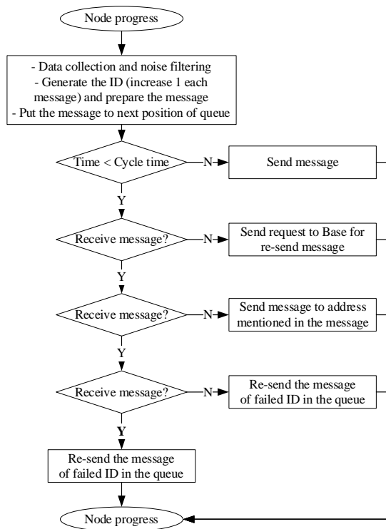
Figure 7. Node general algorithm flowchart
