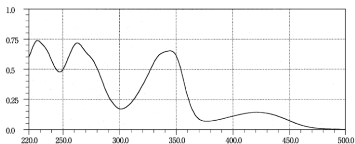
Figure 10. UV-Vis of berberine chloride
