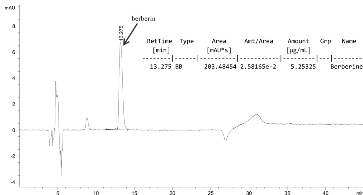
Figure 2. HPLC analysis of berberine, with the mobile phase composed of ACN-H 2 O:0.1% TFA in linear gradient mode over 0-45 minutes, at a flow rate of 1.5 mL/min.
