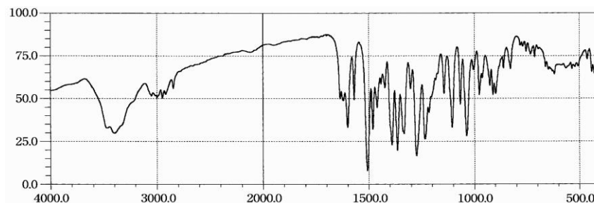
Figure 11. FT-IR of berberine chloride in KBr
