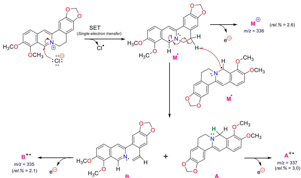
Figure 13. Electron transfer mechanism in the ionization source, \text{M}^+ ( m/z 336), \text{A}^{++} ( m/z 337), and \text{B}^{++} ( m/z 335).
