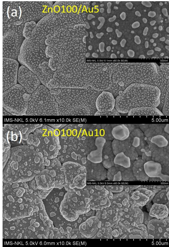
Figure 2. Surface FE-SEM images of Au-decorated ZnO thin films: (a) ZnO100/Au5 and (b) ZnO100/Au10. The insets show corresponding higher-magnification views.
