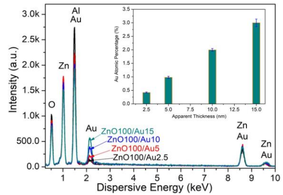
Figure 3. EDS spectra of the ZnO100/Au2.5, ZnO100/Au5, ZnO100/Au10, and ZnO100/Au15 samples. The inset shows the atomic percentage of Au element in the samples versus the nominal thickness.
