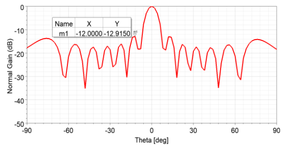
Figure 8. Normal gain of the 1 \times 8 array at 4.9 GHz with an in-phase, equal-magnitude feeding
