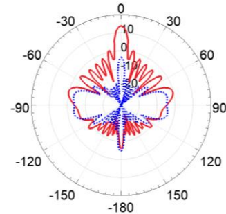
Figure 7. Radiation pattern simulated of 1 \times 8 elements array at 4.9 GHz with an in-phase equal-magnitude feeding (solid line: co-pol, dashed line: cross-pol).
