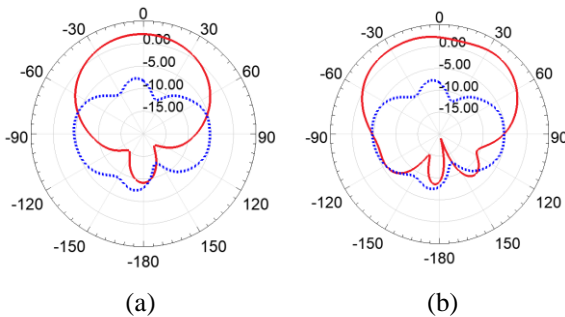
Figure 6. Simulated radiation pattern of the single dipole at 4.9 GHz in (a) x-z plane, (b) y-z plane.
