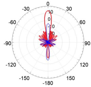
Figure 11. Radiation pattern simulated of 1 \times 8 array at 4.9 GHz (solid line: co-pol, dashed line: cross-pol) with an in-phase trapezoidal feeding
