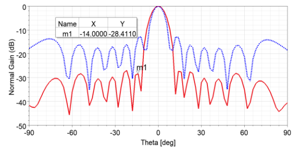
Figure 12. Normal gain of the 1 \times 8 elements array at 4.9 GHz with an in-phase trapezoidal feeding
