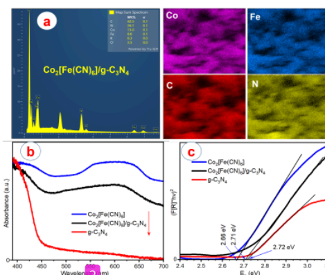
Figure 3. (a) Elemental mapping images of Co, Fe, C, and N for the \text{Co}_2[\text{Fe}(\text{CN})_6]/\text{g-C}_3\text{N}_4 composite, (b) UV-Vis DRS spectra and (c) band gap energy of the materials
