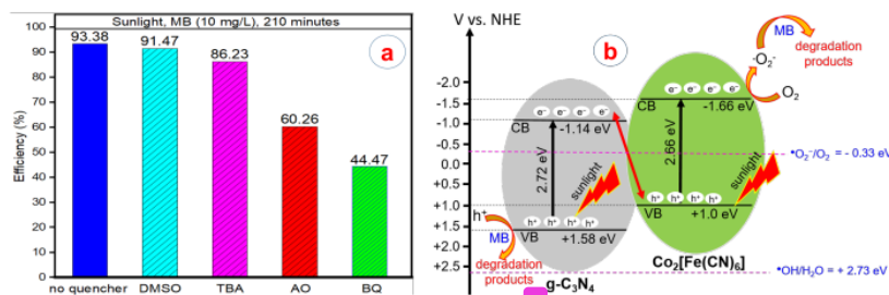
Figure 5. (a) Photocatalytic degradation of MB on Co 2 [Fe(CN) 6 ]/g-C 3 N 4 in the presence of various scavengers, and (b) Proposed Z-scheme mechanism for the photocatalytic activity of the Co 2 [Fe(CN) 6 ]/g-C 3 N 4 composite
