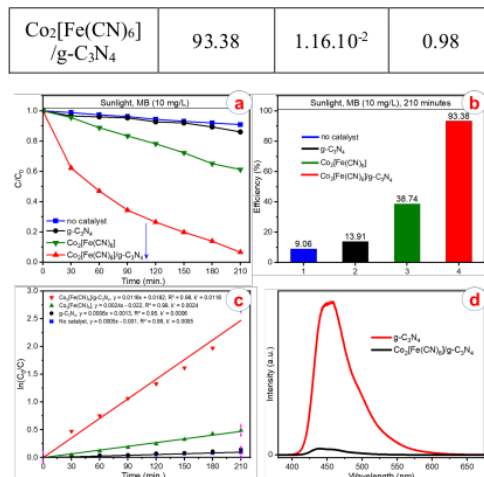
Figure 4. (a→c) Photocatalytic degradation of MB over \text{Co}_2[\text{Fe}(\text{CN})_6] , \text{g-C}_3\text{N}_4 , and \text{Co}_2[\text{Fe}(\text{CN})_6]/\text{g-C}_3\text{N}_4 ; (d) PL spectra of the corresponding materials
