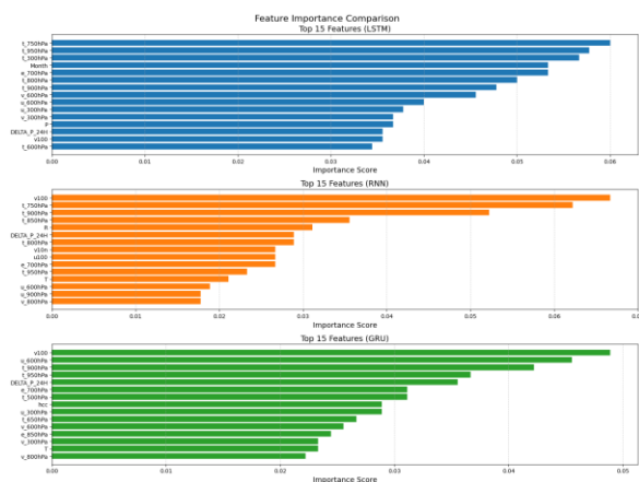
Figure 9. Importance of Features.
