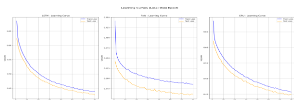
Figure 8. Training progress and loss log for LSTM, RNN, and GRU.
