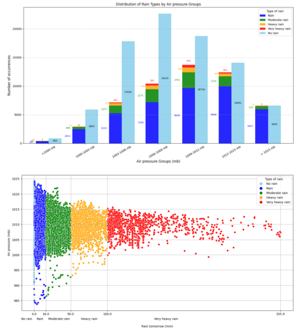
Figure 5. Distribution of rainfall types by pressure group.
