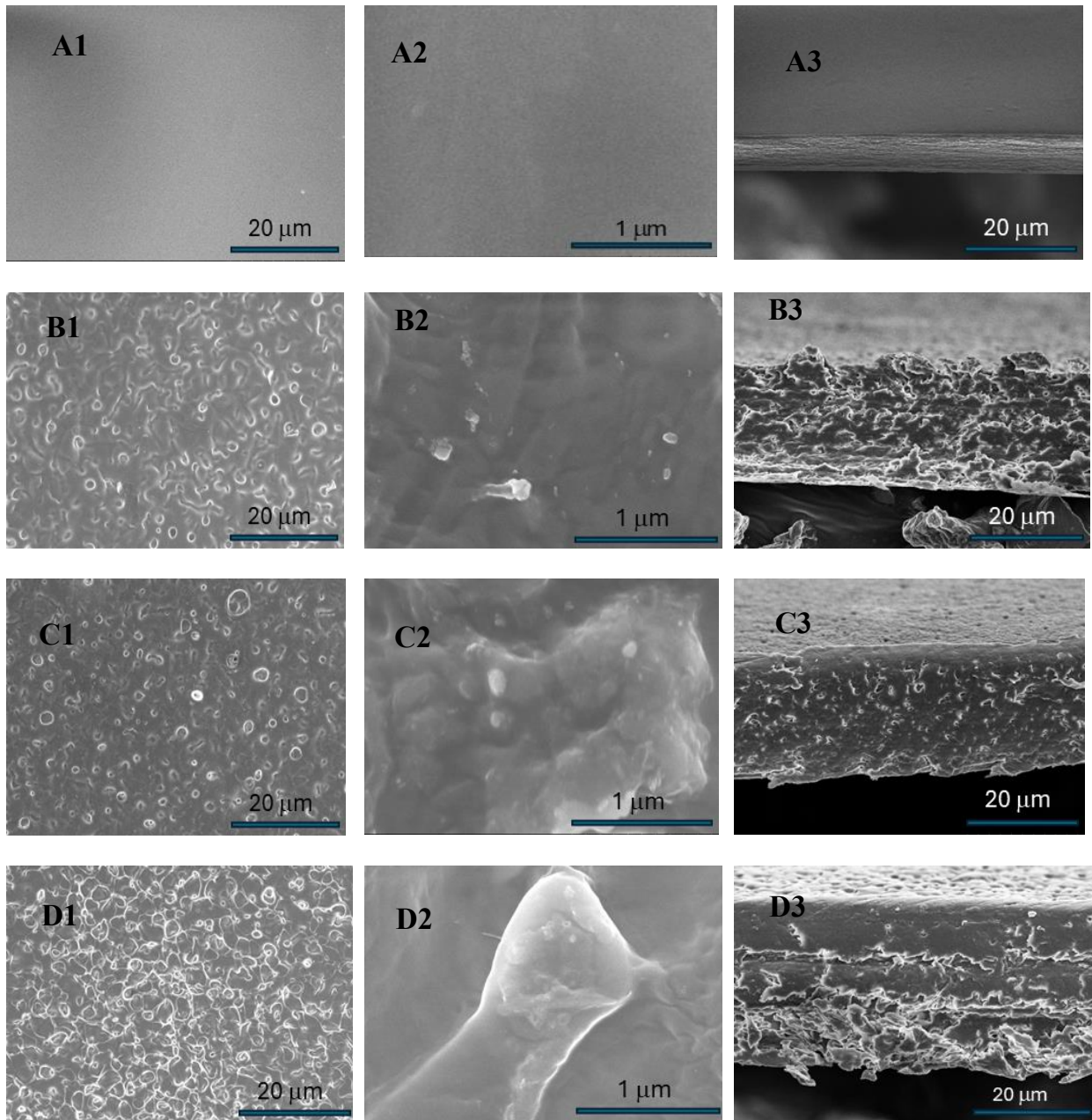
Figure 2. SEM images of surface (1, 2) and cross-section (3) of active films: (A1, A2, A3) CA/SA/OEO 0%; (B1, B2, B3) CA/SA/OEO 3%; (C1, C2, C3) CA/SA/OEO 4.5%; (D1, D2, D3) CA/SA/OEO 6%
