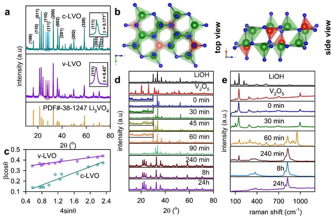
Figure 1. (a) XRD patterns of the c-LVO and v-LVO (the insets are the enlargement of XRD patterns in 2\theta -range of 31-34°; (b) the illustration of top and side views of orthorhombic \text{Li}_3\text{VO}_4 , where red, green, and blue represent vanadium, lithium, and oxygen; (c) Williamson-Hall plots of c-LVO and v-LVO; (d) ex-situ XRD and (e) ex-situ Raman spectroscopy of the LiOH, \text{V}_2\text{O}_5 , and v-LVO after various reaction times from 0 min to 24 hours.
