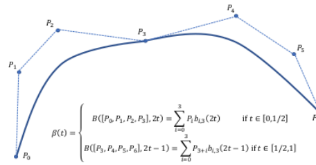
Figure 2. A two-piece cubic Bézier curve
