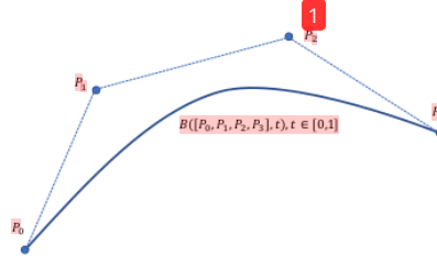
Figure 1. A cubic Bézier curve
