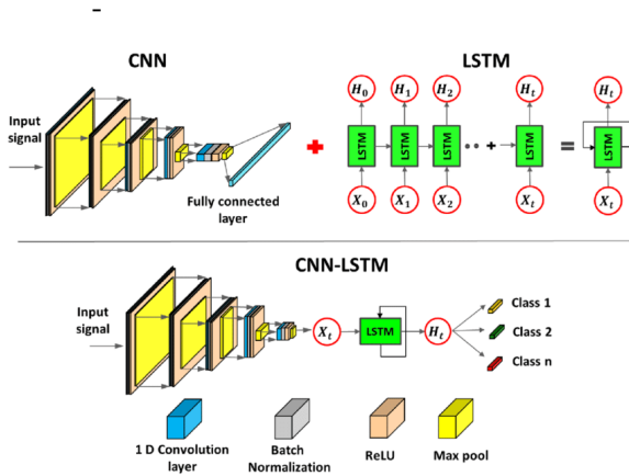
Figure 1. Overall architecture diagram of the hybrid CNN-LSTM model
