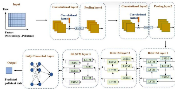
Figure 1. Overall architecture diagram of the hybrid CNN-BiLSTM model
