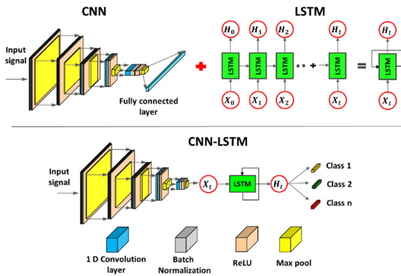
Figure 1. Overall architecture diagram of the hybrid CNN-LSTM model
