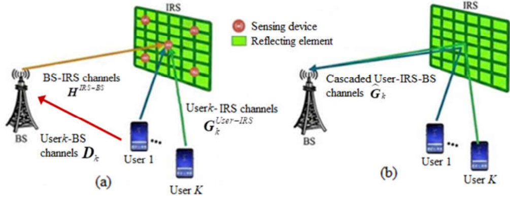
Figure 2. Illustration of separate channel estimation for semi-passive IRSs (a) and cascaded channel estimation (uplink) for fully passive IRSs (b).
