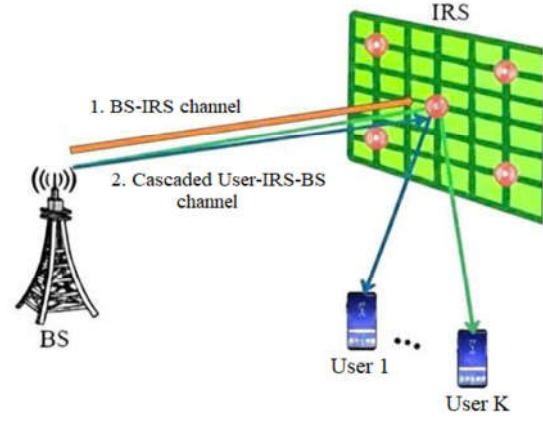
Figure 4. Hybrid or combined framework integrating individual-channel estimation and cascaded channel estimation.
