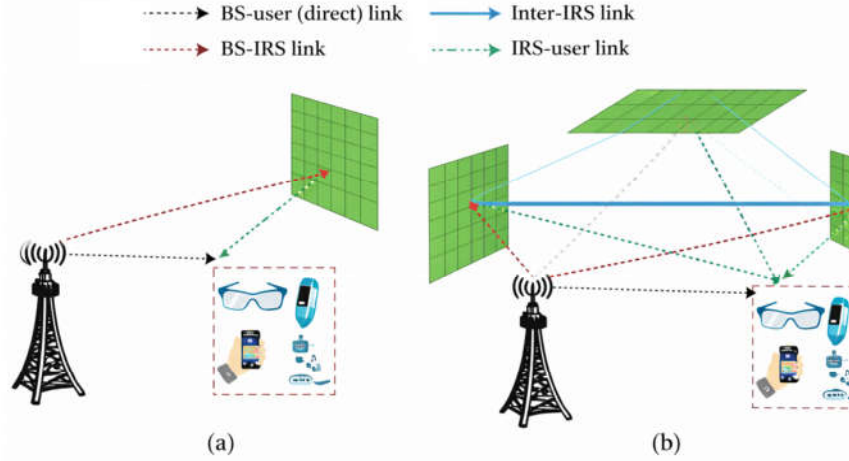
Figure 6. IRS-aWC system with different IRS deployments:
