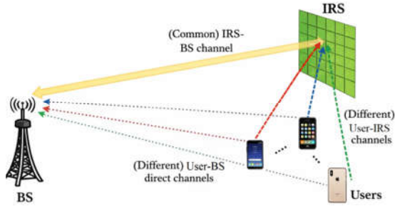
Figure 5. Uplink channel estimation in IRS-aided multi-User wireless communication systems.
