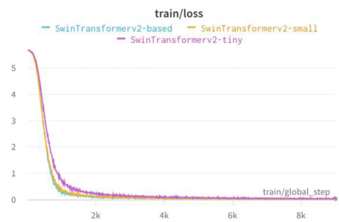
(a) The loss of three models on the training set
