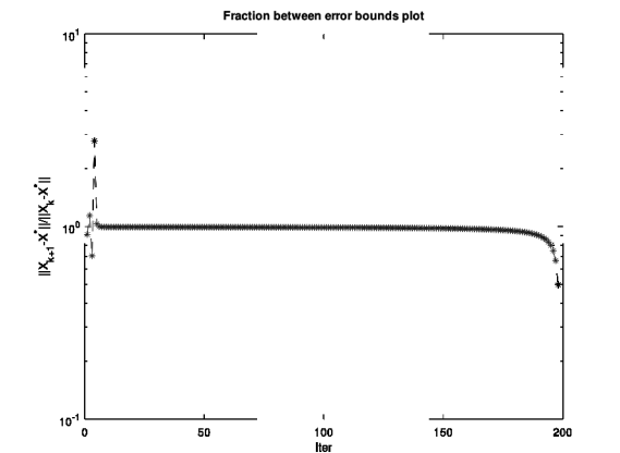
Figure 3. Superlinear convergence of Algorithm 2 with snopt solver
