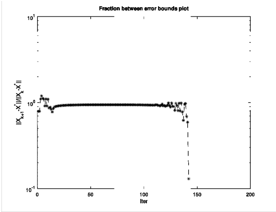
Figure 2. Superlinear convergence of Algorithm 2 with minos solver
