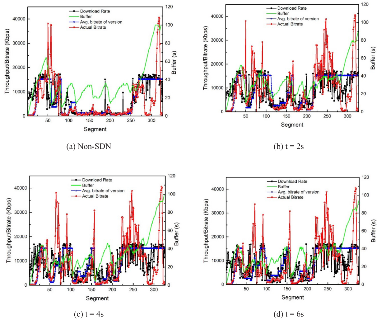
Figure 6. Result of Non-SDN case (a) and Results of Periodical Routing with SDN case (b, c, d).
