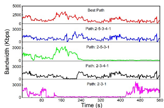
Figure 5. Experimental bandwidths
