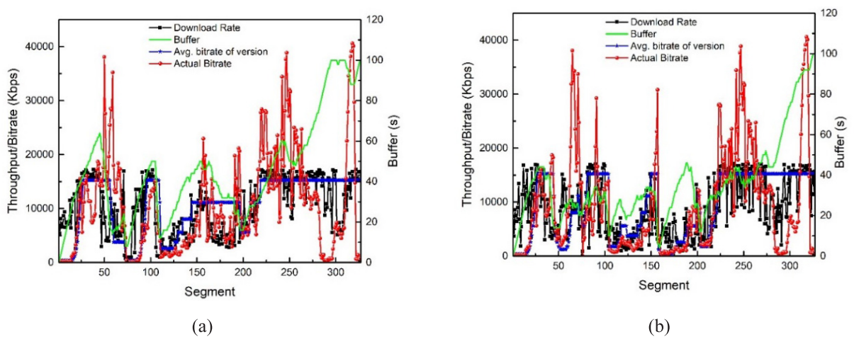
Figure 7. Results of Adaptive Routing without (a) and with (b) monitoring.
