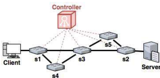
Figure 4. Experimental network topology.
