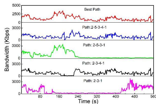
Figure 5. Experimental bandwidths.
