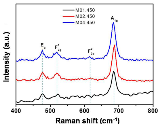
Figure 7. Raman spectra of samples synthesized at different \text{Co}(\text{NO}_3)_2 \cdot 6\text{H}_2\text{O} concentrations and calcination temperature of 450^\circ\text{C} (M01.450, M02.450, and M04.450).
