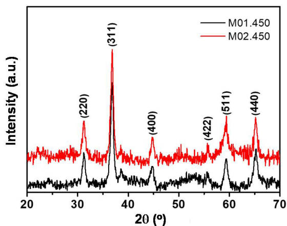
Figure 6. The XRD patterns of \text{Co}_3\text{O}_4 IO at calcination temperature of 450^\circ\text{C} and \text{Co}(\text{NO}_3)_2 \cdot 6\text{H}_2\text{O} concentrations of 0.1 M and 0.2 M.
