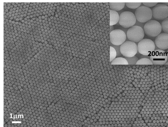
Figure 2. SEM image of PS beads deposited on glass substrate (the inset is the enlarged image of corresponding sample).
