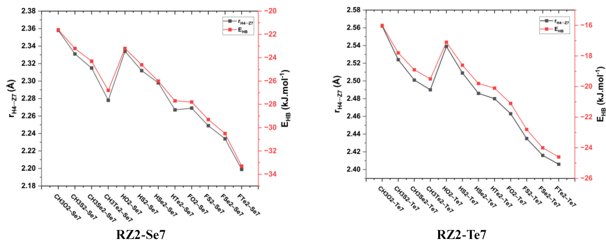
Figure S1b. The relationship between the H4...Z7 interaction distance and individual energy ( E_{HB} ) of O-H...Z7 hydrogen bond in RZ2-Z7 complexes (with R= H, F, CH 3 ; Z2(Z7) = O, S, Se, Te).
