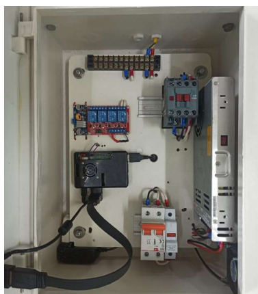
Figure 10. Experimental model of control center.
