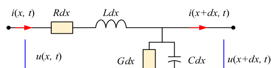
Figure 3. Single-phase transmission line model of distributed parameters.
