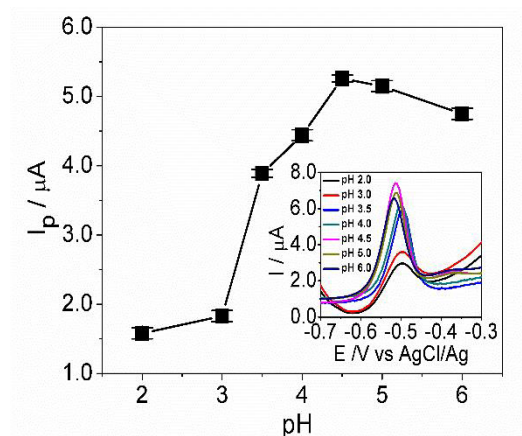
Figure 3. Effects of pH value on the peak current of 10 \mu\text{g.L}^{-1} Pb(II) in an acetate buffer solution.
