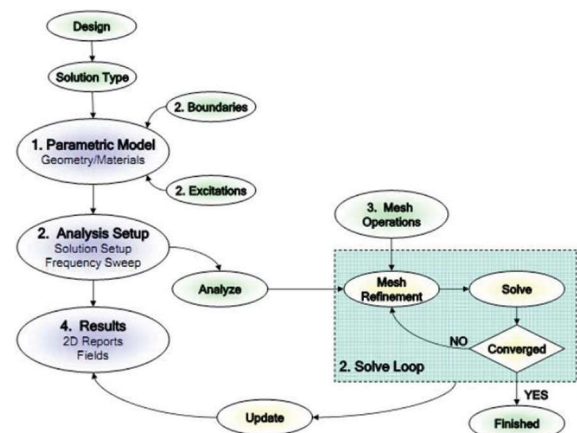
Figure 3. The process of solving the problem using the Finite Element method
