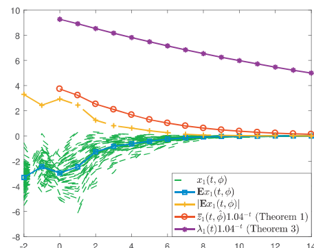
Figure 1. Trajectories of x_1(t, \phi) , the mean value \mathbb{E}x_1(t, \phi) and its \alpha -exponential mean estimates
