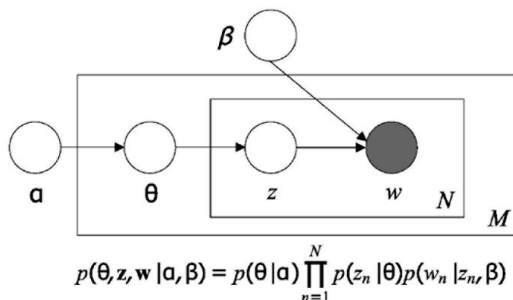
Figure 1. Latent Dirichlet Allocation model. 14
