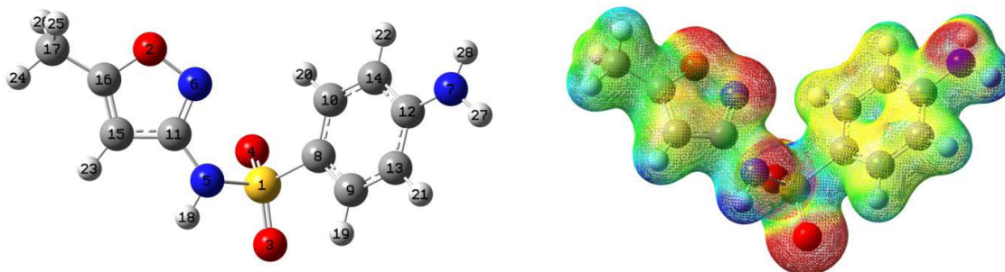
Figure 2. The optimized geometry and MEP map of sulfamethoxazole at B3LYP/6-31G(d,p) level (electron density = 0.02 au; region of -5.10 -5 to 0.20 au)
