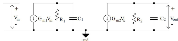
Figure 4. Small-signal model op-amp without compensation
