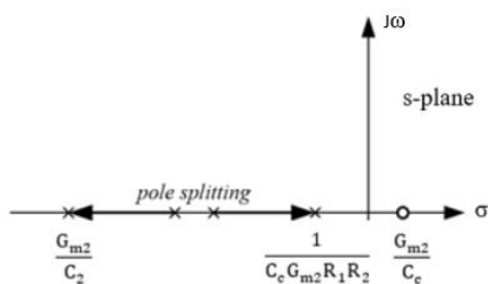
Figure 6. Pole/zero locations
