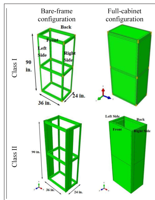
Figure 9. Cabinet models proposed, adapted from Lim. 18
