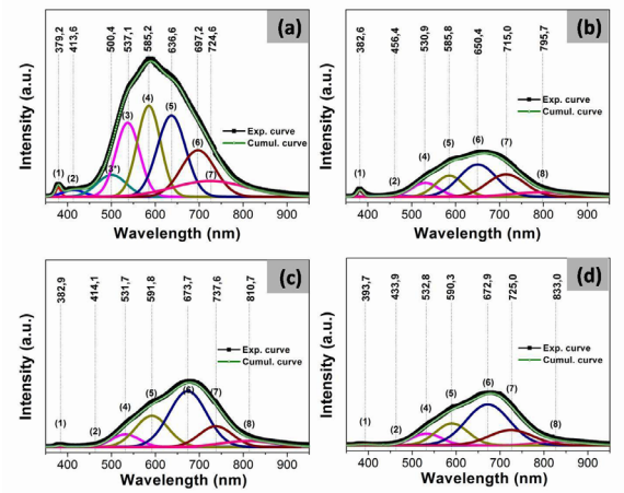
Figure 5. PL spectrum of ZnO (a), NiO(2)/ZnO (b), NiO(8)/ZnO (c) and NiO(16)/ZnO (d) materials.
