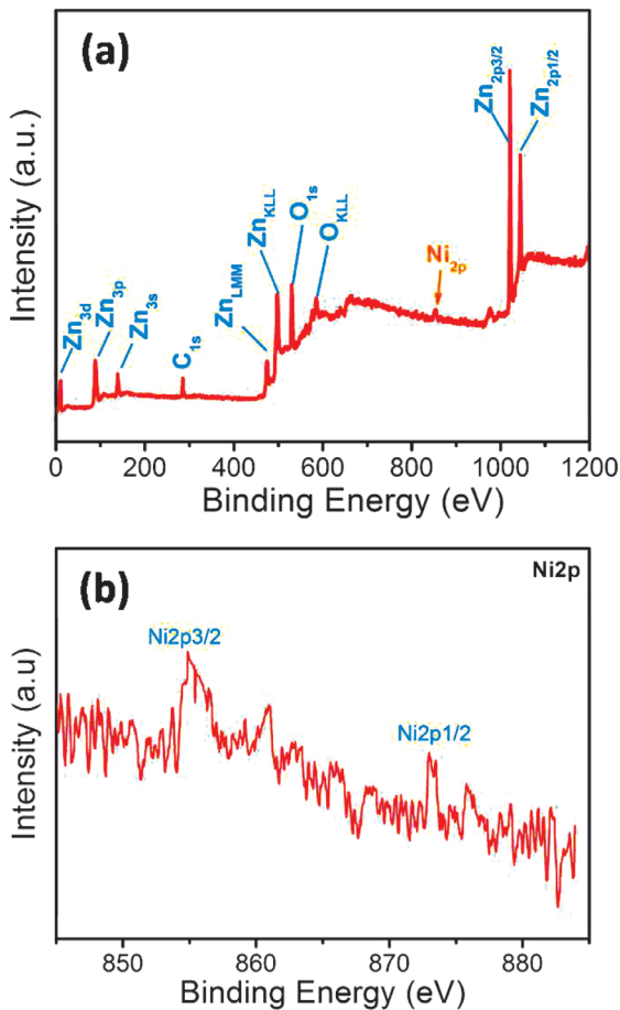
Figure 3. The total XPS spectrum (a) and high manification of Ni2p (b) in NiO(16)/ZnO structure.
