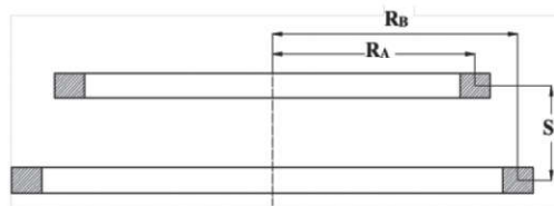
Figure 8. Cross section of two coaxial rings
