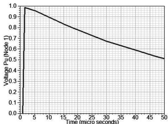
Figure 17. Voltage values at node 1 - Interleaved disk winding
