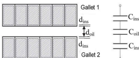
Figure 6. Capacitance between two galleys
