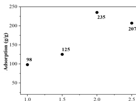
Figure 5. Results of the influence of KPS concentration on water adsorption of O-CMCS-SAP.
