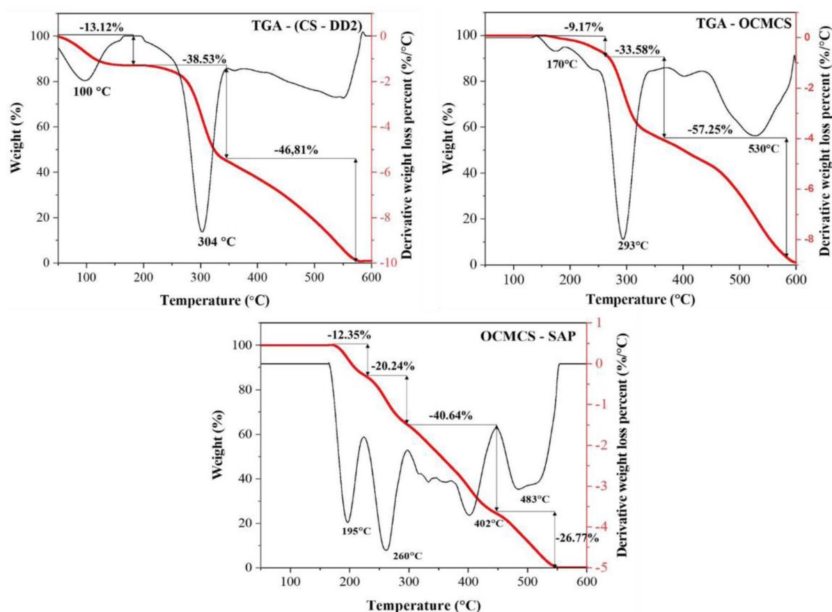
Figure 14. TGA results of CS-DD2, O-CMCS, and O-CMCS-SAP.
