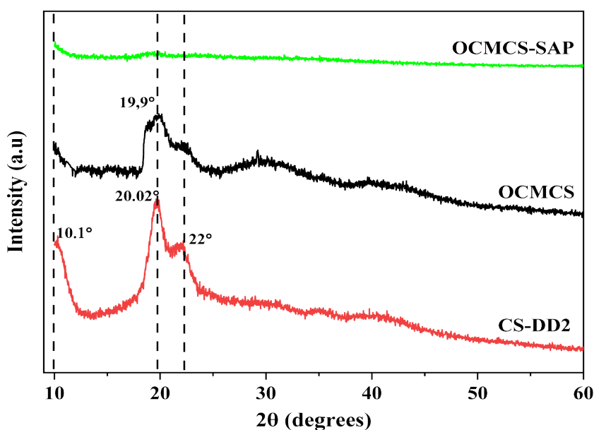
Figure 13. XRD spectra of CS-DD2, O-CMCS, and O-CMCS-SAP.
