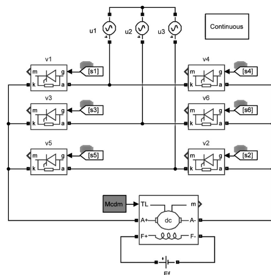
Figure 3. Circuit diagram of T-D drive system.
