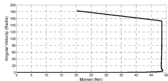
Figure 6. Characteristic of DCM in CLPWM-DCM system when the motoring mode happens
