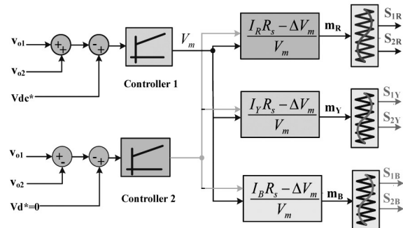
Figure 2. Control circuit diagram of PWM rectifier. 11,12
