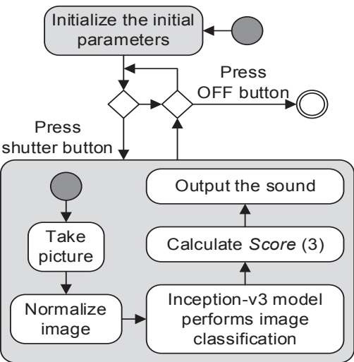
Figure 10. State diagram for recognizing objects.
