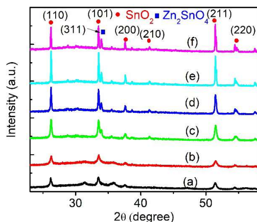
Figure 1. XRD patterns of \text{SnO}_2\text{-Zn}_2\text{SnO}_4 sample unannealed (a) and annealed at different temperature of 500^\circ\text{C} (b); 900^\circ\text{C} (c); 1000^\circ\text{C} (d); 1100^\circ\text{C} (e) and 1200^\circ\text{C} (f).
