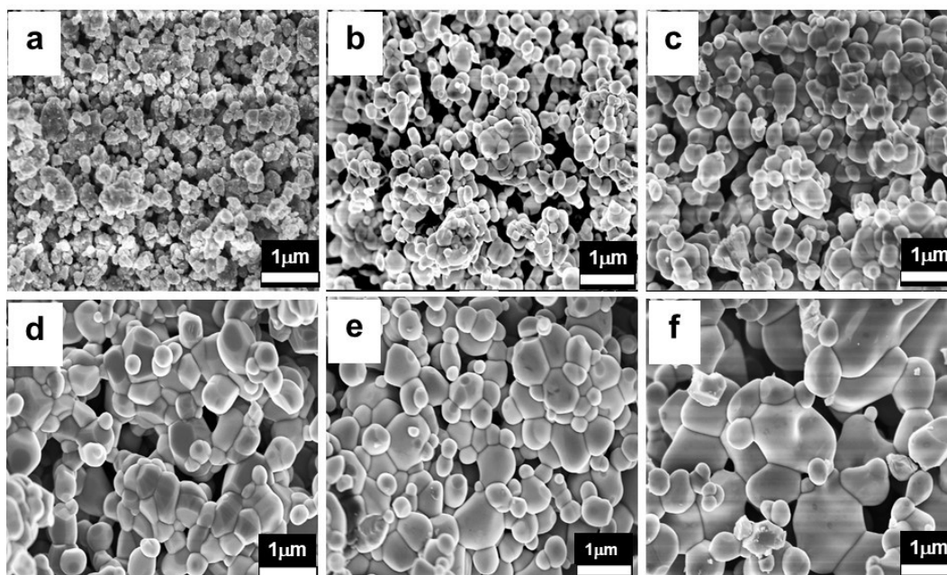
Figure 2. FESEM images of \text{SnO}_2\text{-Zn}_2\text{SnO}_4 sample: unannealed (a) and annealed at different temperature of 500^\circ\text{C} (b); 900^\circ\text{C} (c); 1000^\circ\text{C} (d); 1100^\circ\text{C} (e) and 1200^\circ\text{C} (f).
