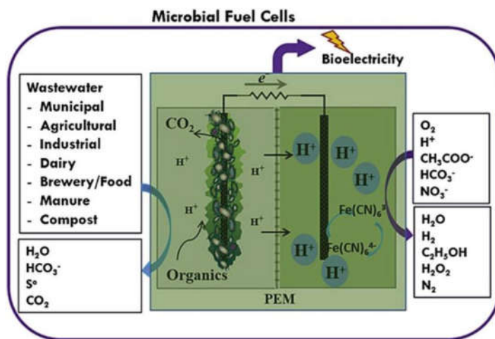
Figure 1. Structure diagram of microbial fuel cell. 15
