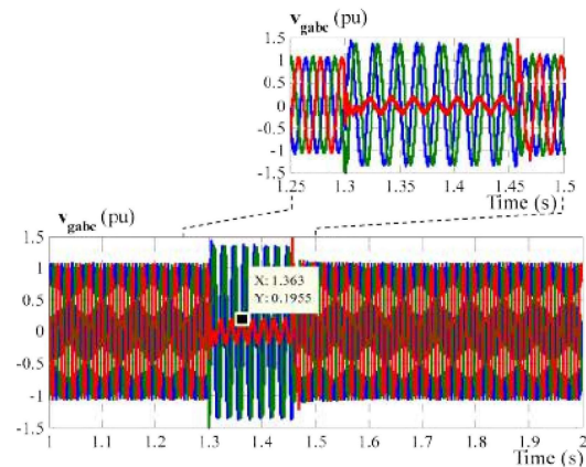
Figure 15. The grid voltage with 2 nd case study.
