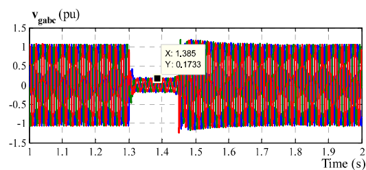
Figure 12. The grid voltage with 1 st case study.
