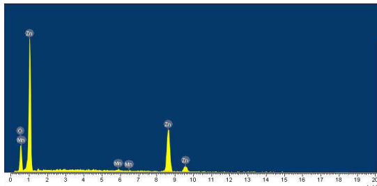
Figure 6. EDS spectra of Mn-doped (1% mol) ZnO nanoparticles.
