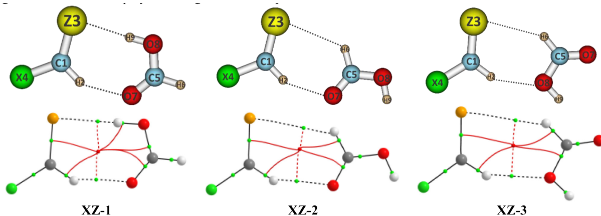
Figure 1. The stable structures and topological features of \text{XCHZ} and \text{HCOOH} complexes ( \text{X} = \text{H}, \text{F}, \text{Cl}, \text{Br}, \text{CH}_3, \text{NH}_2 and \text{Z} = \text{Se}, \text{Te} ).
