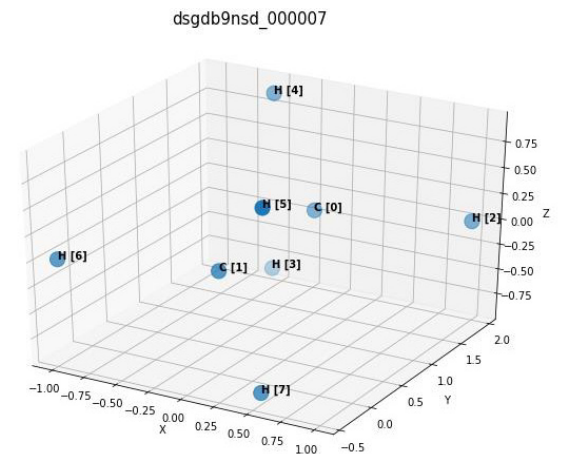
Figure 2. Eight atoms of the molecule dsgdb9nsd_000007 in the XYZ cartesian coordinate system.
