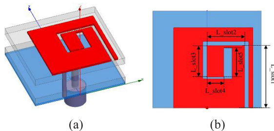
Figure 10. Geometry of the proposed dual-band PIFA: (a) Perspective view, (b) Top view.
