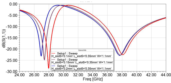
Figure 15. Simulated S_{11} of the antenna versus different values of H_{\text{slot5}} .
