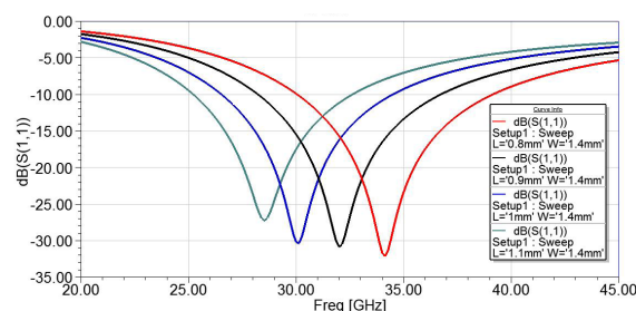
Figure 4. Simulation results of S11 of the single band PIFA with the various values of L .
