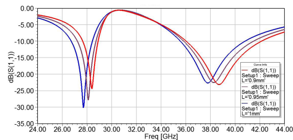
Figure 13. Simulated S11 versus different values of L.
