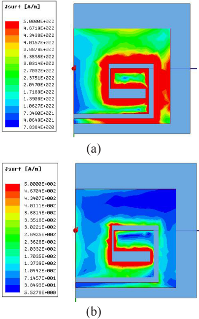
Figure 17. Current distribution on the dual-band PIFA antenna at: (a) 28 GHz, (b) 38 GHz.
