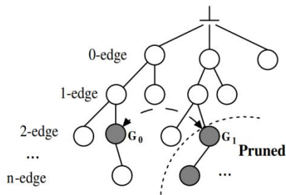
Figure 3. DFS code tree 3
