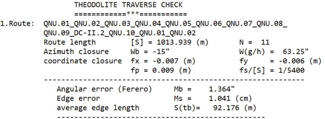
Figure 1. Result of control network summary
