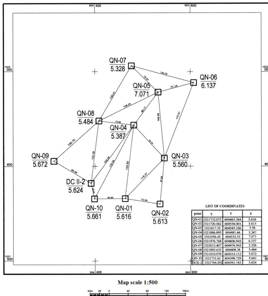
DIAGRAM OF THE COORDINATE CONTROL NETWORK QUY NHON UNIVERSITY
