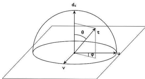
Figure 3. Space for generating reflection rays
