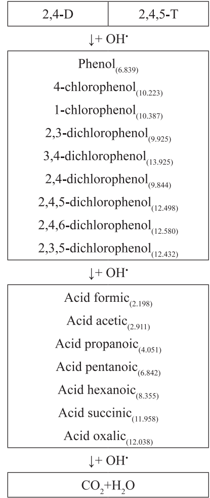
Figure 9. Model of 2,4-D or 2,4,5-T decomposition by DC high voltage with electrochemical plasma
