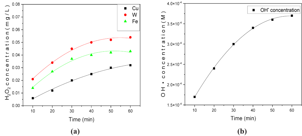
Figure 7. The dependence of the electrochemical plasma lifetime of the H_2O_2 concentration formed at 15 kV, 30°C, D_{A-C} 200 mm on the W, Cu, Fe (a) electrodes as well as the OH^\bullet free radical concentration on the Fe electrode (b).
