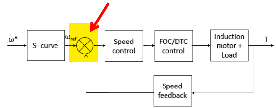
Figure 2. Speed control model with integrated S-curve acceleration profile
